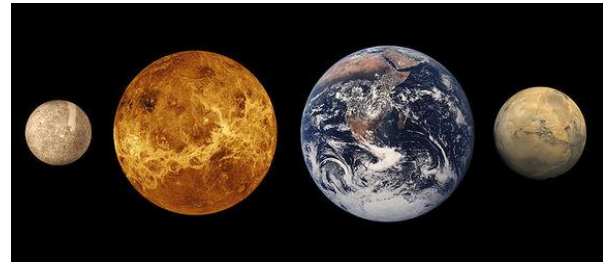
Inner Planets
