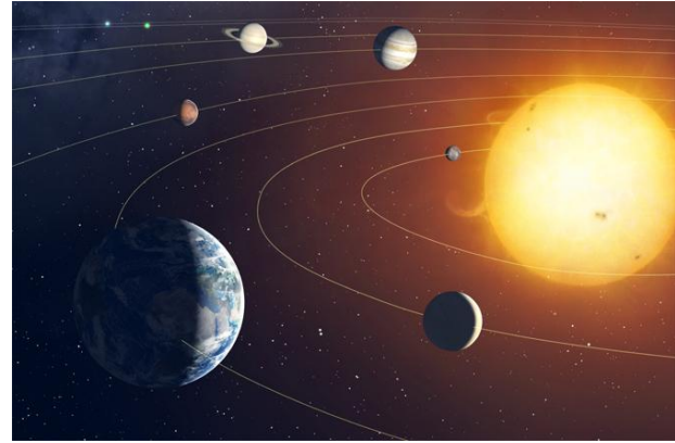
Solar System
