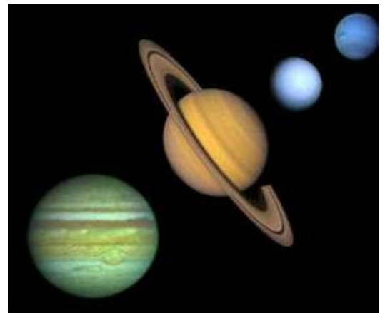
Outer Planets
